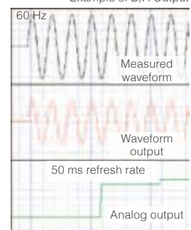
Example of D/A Output
