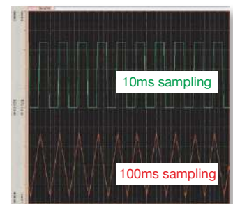
Measurement comparison of 5 Hz square pulse waveform with 10 ms (upper trace) and 100 ms sampling (using the supplied Logger Utility program)
